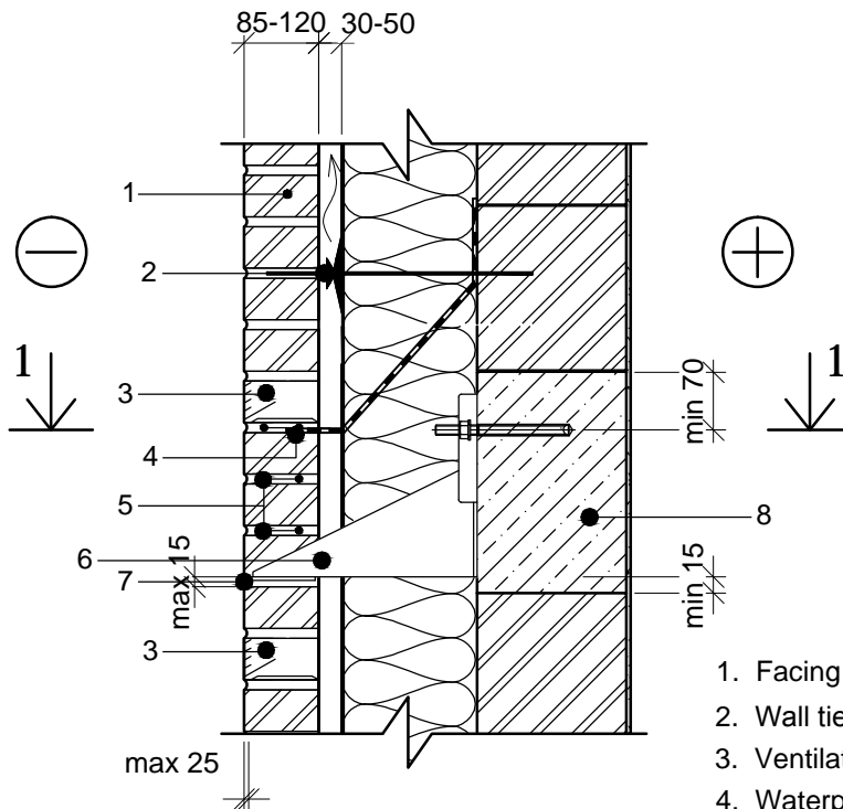
SECTION 1-1
