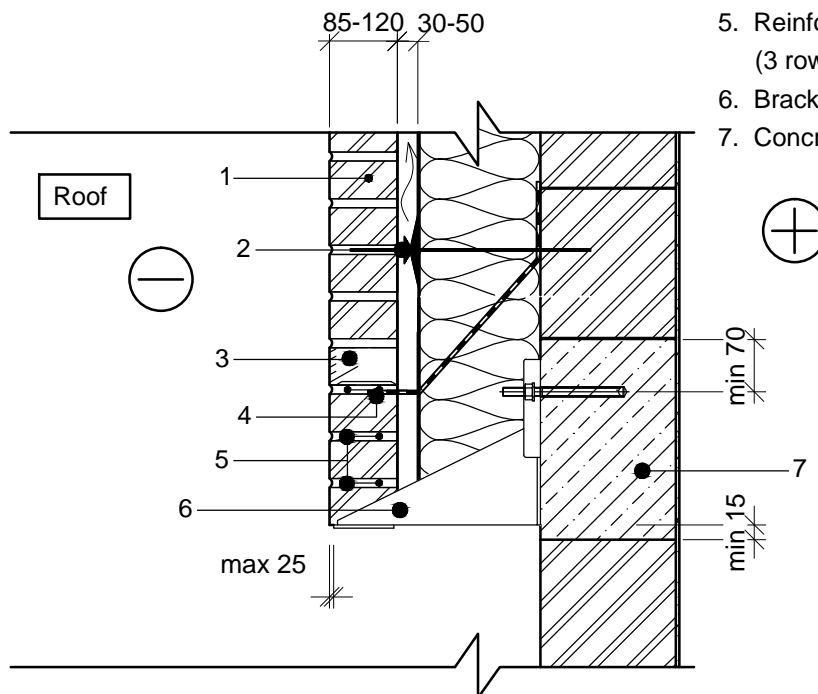
SECTION 1-1
