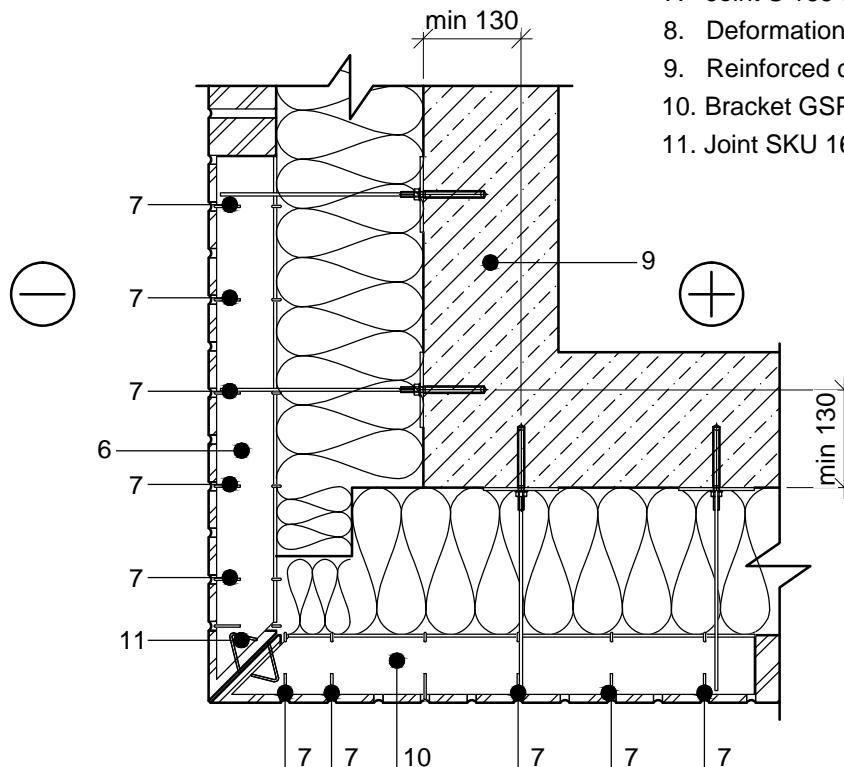
SECTION 1-1
