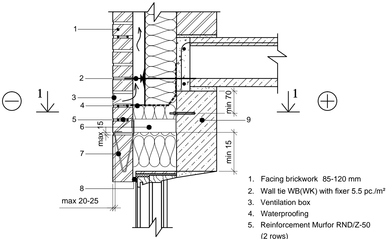
SECTION 1-1
