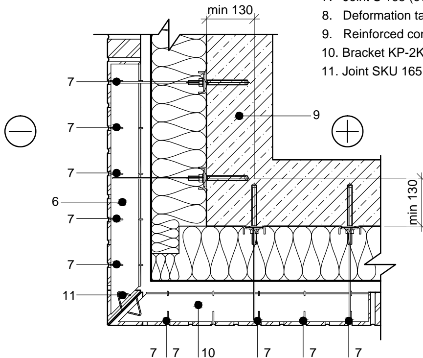
SECTION 1-1
