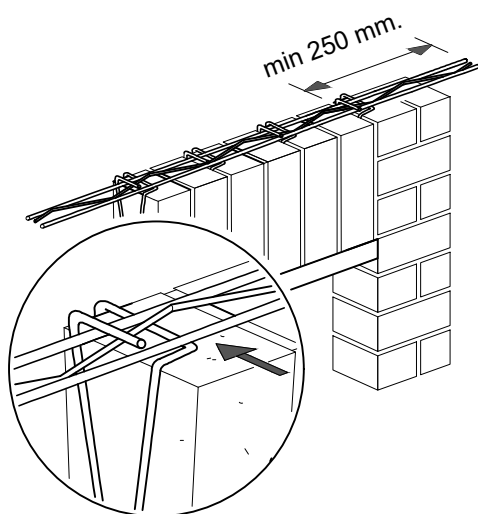
Reinforcement Murfor RND/Z-50 is inserted through grooves of lintel hooks. Reinforcement rods extend beyond the opening edges by at least 250 mm in both sides
