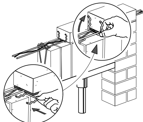
Lintel hooks SU 50-45 in every second vertical joint of the second course
