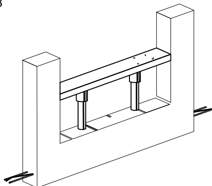
Construction of formwork
