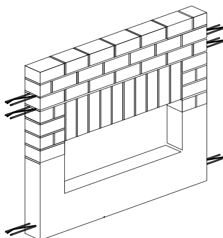
Formwork should be dismantled after 2 weeks
