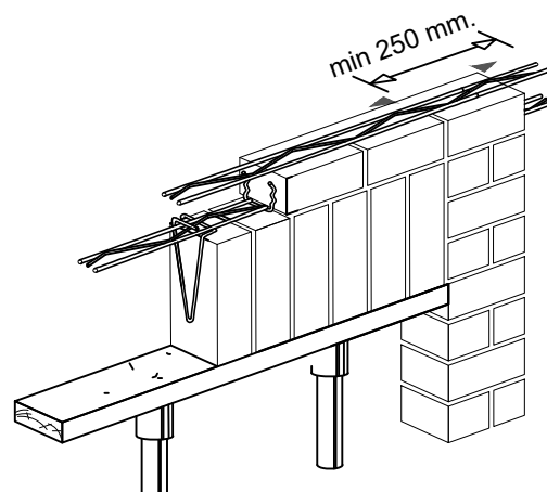
Reinforcement Murfor RND/Z-50 in the second course of brickwork. Further throughout the height, 1 reinforcement rod at every 300...500 mm
