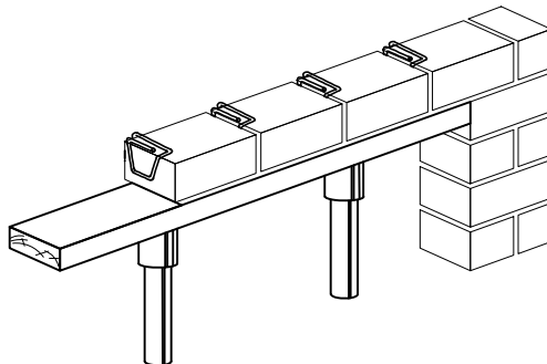
Lintel hooks SK 50-40 in every vertical joint of the first course
