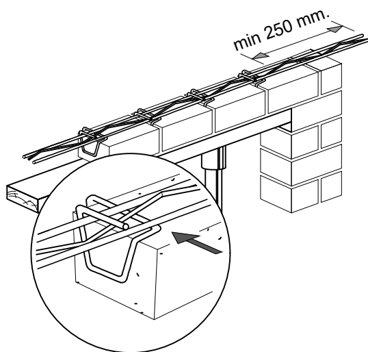
Reinforcement Murfor RND/Z-50 is inserted through grooves of lintel hooks. Reinforcement rods extend beyond the opening edges by at least 250 mm in both sides
