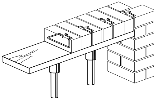
Lintel hooks SKK 50-65 should be placed into the mortar, in every second vertical joint of the first row of brickwork
