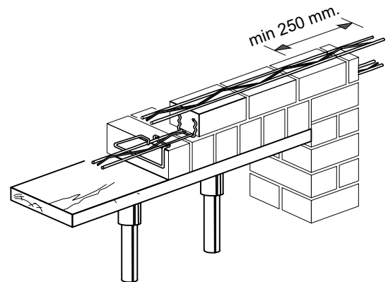
Reinforcement Murfor RND/Z-50 in the second course of brickwork. Further throughout the height, 1 reinforcement rod at every 300...500 mm
